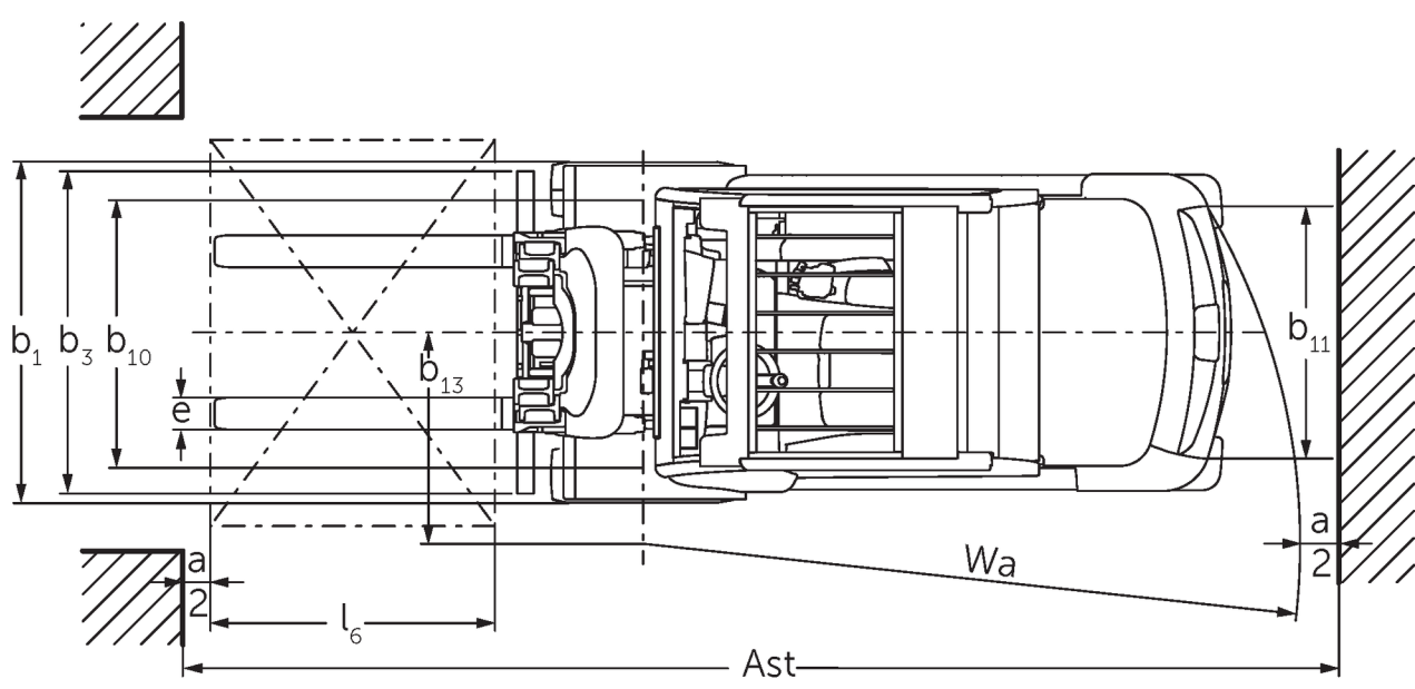
Technical drawing EFG 5 (2015)
